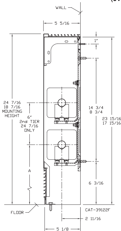
JVB/VB-AR18 24EI (JVB Shown)
